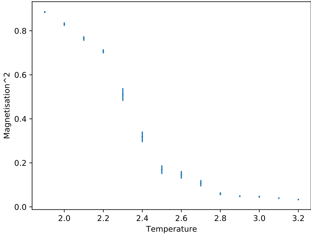
Magnetisation 2 , Metropolis
