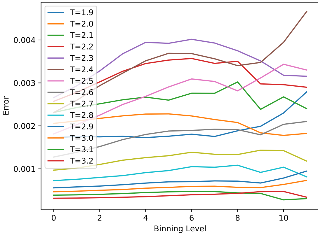
Binning analysis Wolff, magnetisation
